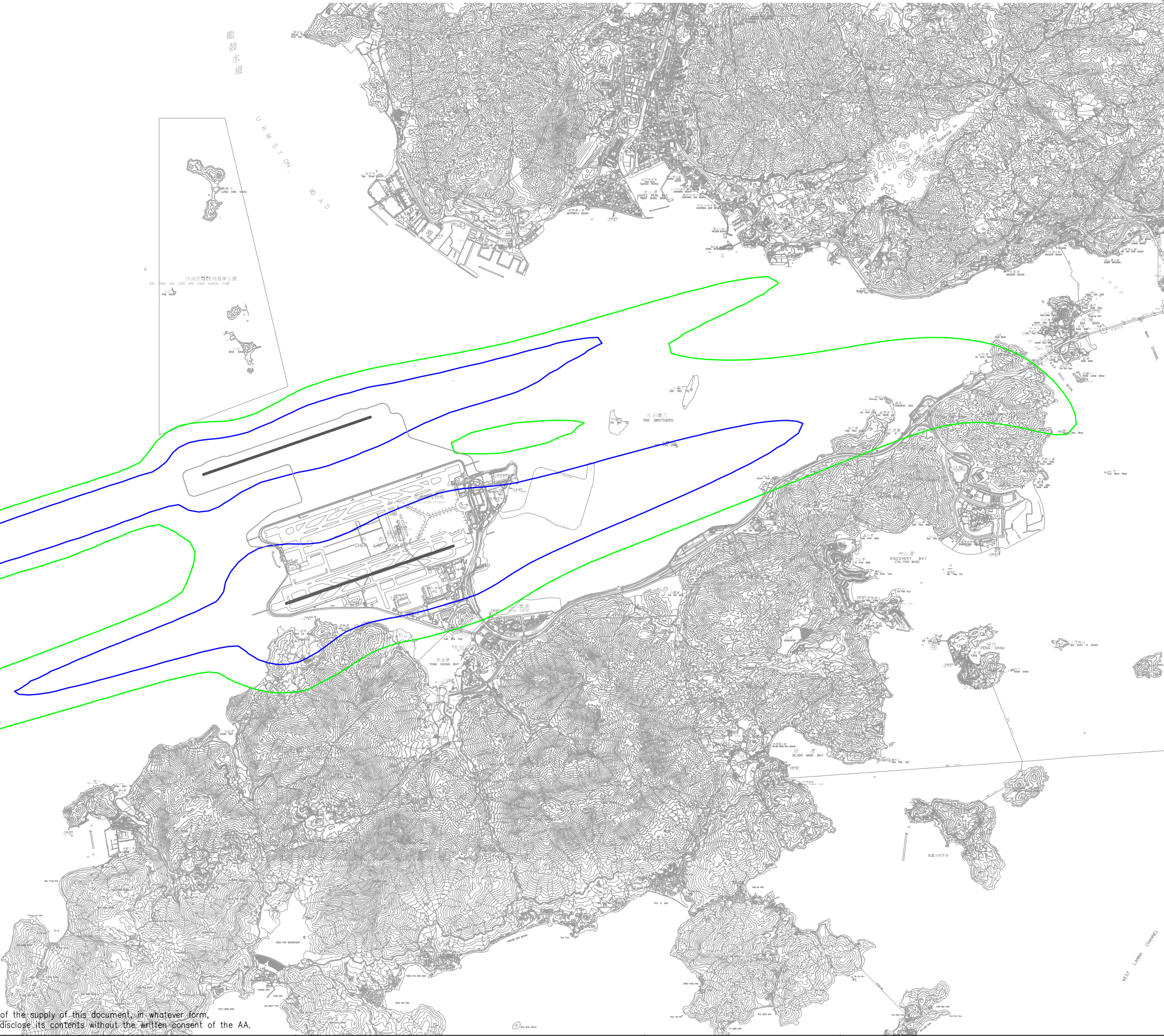
Figure 4.2 NEF Contours for Interim Phase Scenario in Approved 3RS EIA Report
