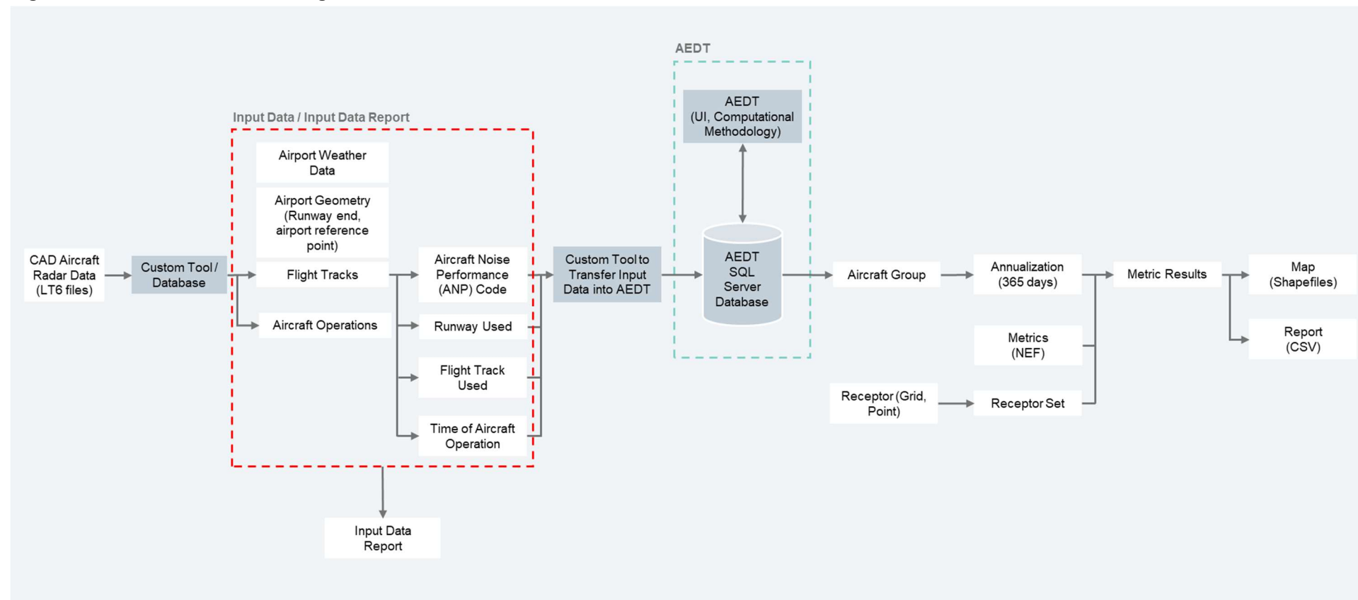
Figure 3.1: Aircraft Noise Modelling Process
